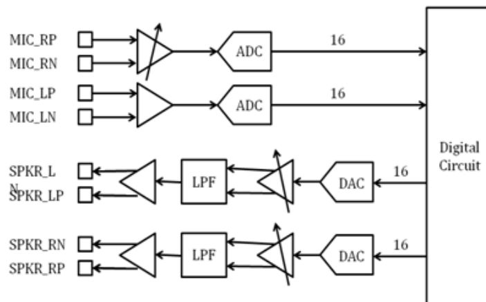
Figure 3-1: Audio Diagram
