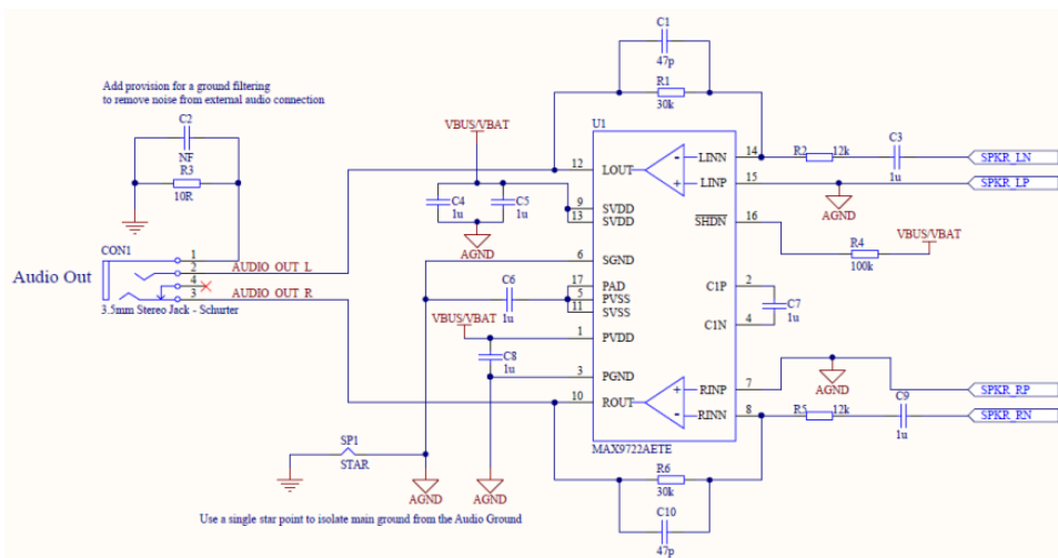
Figure 4-10: Isolation
