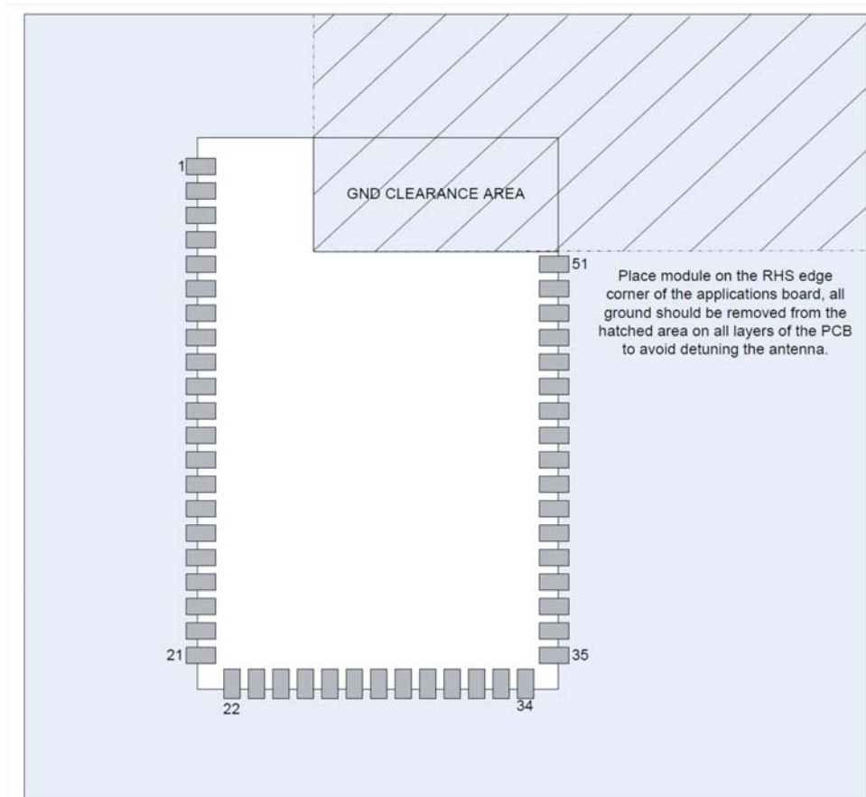
Figure 2-2: Placement Layout
