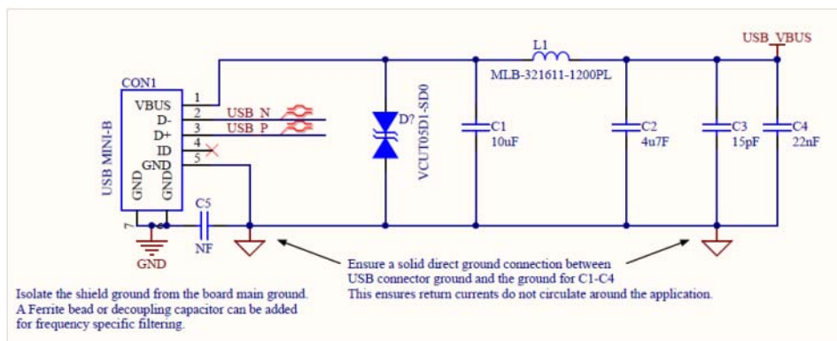
Figure 4-6: Example USB Supply Configuration
